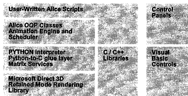
Figure 4: The Alice Software Architecture. User scripts are written in Python as is much of the Animation Engine Layer beneath it. The layers below this are written in C. Alice includes a separate Control Panels facility for creating Visual Basic GUI components directly through the Python scripting language.
